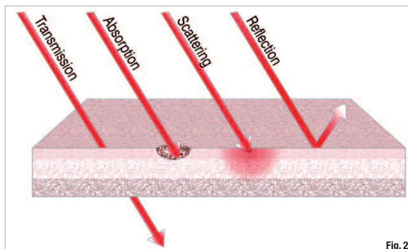
Fig. 2_Laser-tissue interaction.
